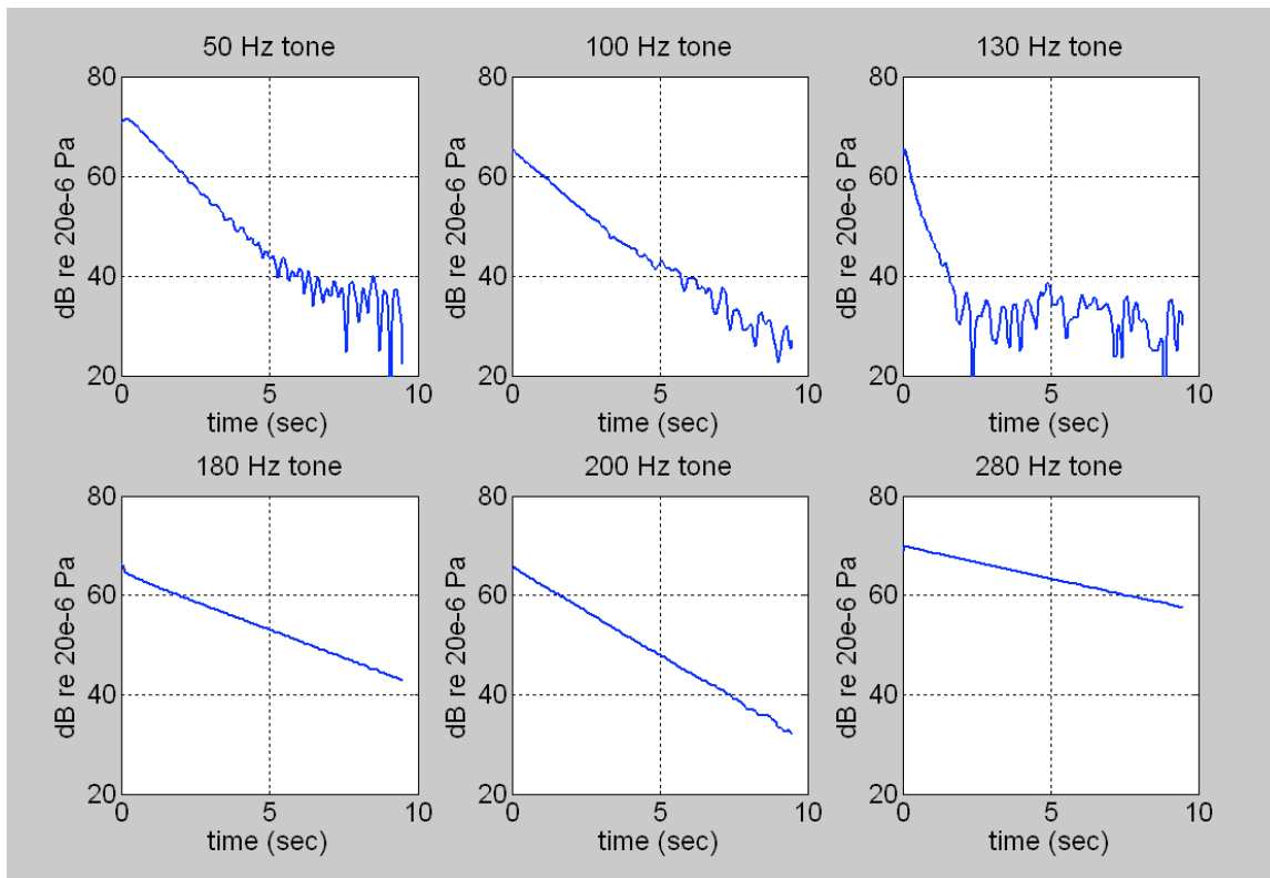
Figure 5.24 Individual learning curves for tones in noise signal for ANC with EE-FXLMS algorithm using 256-coefficient genetic Sys ID model and weighted reference.
