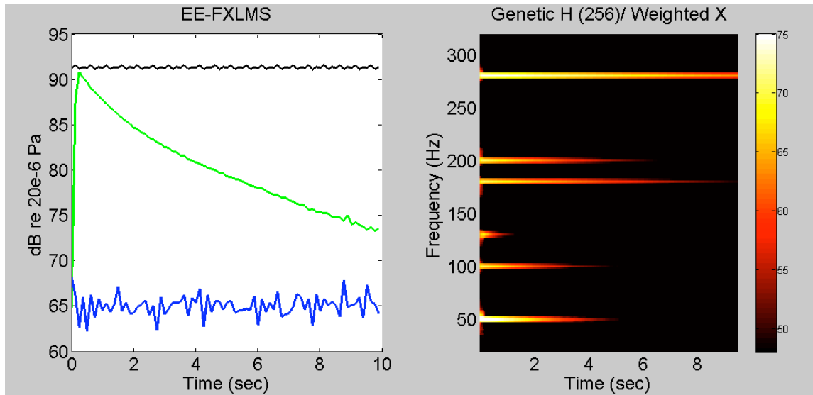
Figure 5.23 Plot of three time captures (left) and spectrogram of converging error signal from the time ANC was enabled (right) for ANC test with EE-FXLMS algorithm using 256-coefficient genetic Sys ID model and weighted reference.
