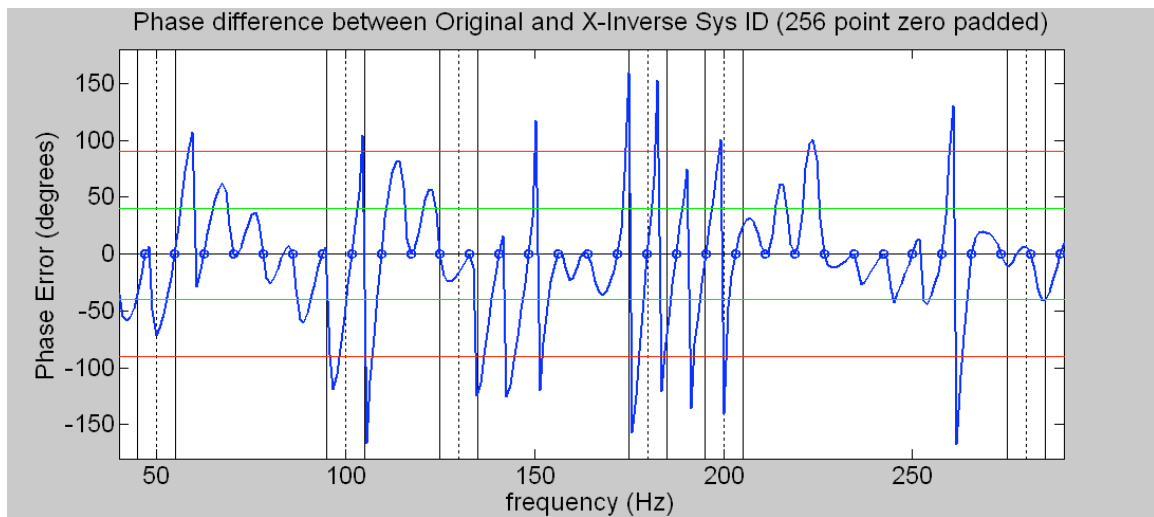
Figure 5.20 Phase Errors (difference from original) for the 256-coefficient x-inverse Sys ID model. Dashed vertical lines mark tonal frequencies and solid vertical lines mark \pm 5 Hz around those tonal frequencies. Note that the phase error exceeds 40^\circ (green horizontal lines) at the 50 and 100 Hz and approaches the 90^\circ degree stability limit (red line) at 200 Hz.
