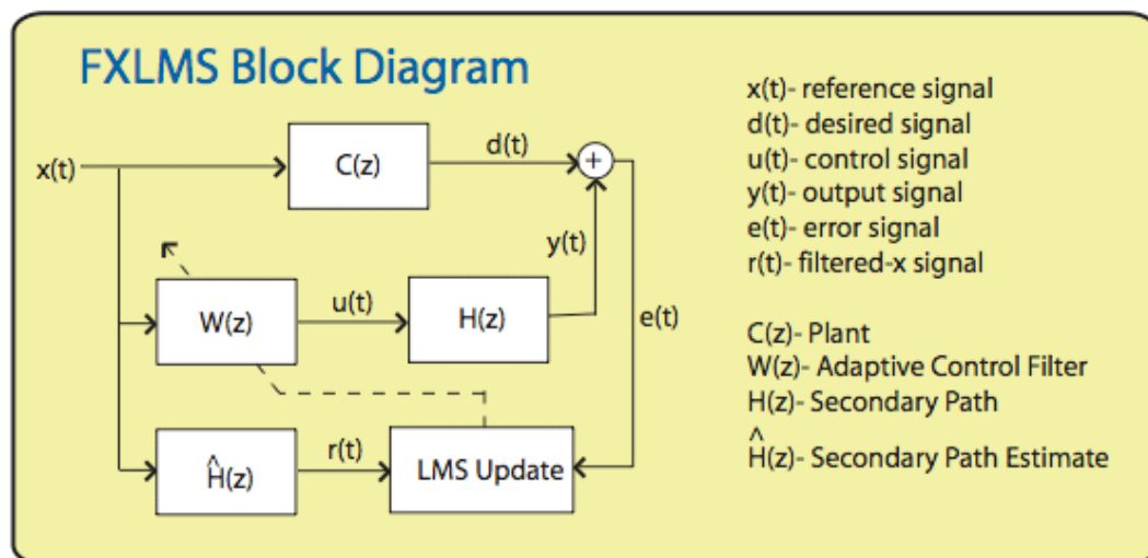
Figure 2.1 Block diagram of the filtered-x least mean square algorithm.
